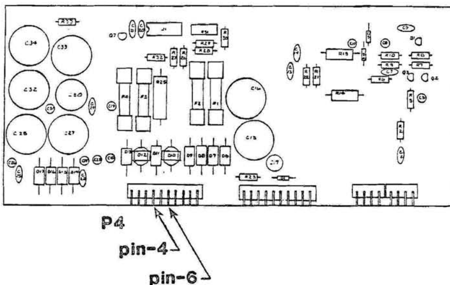
G-80 Power Supply PC Assembly
