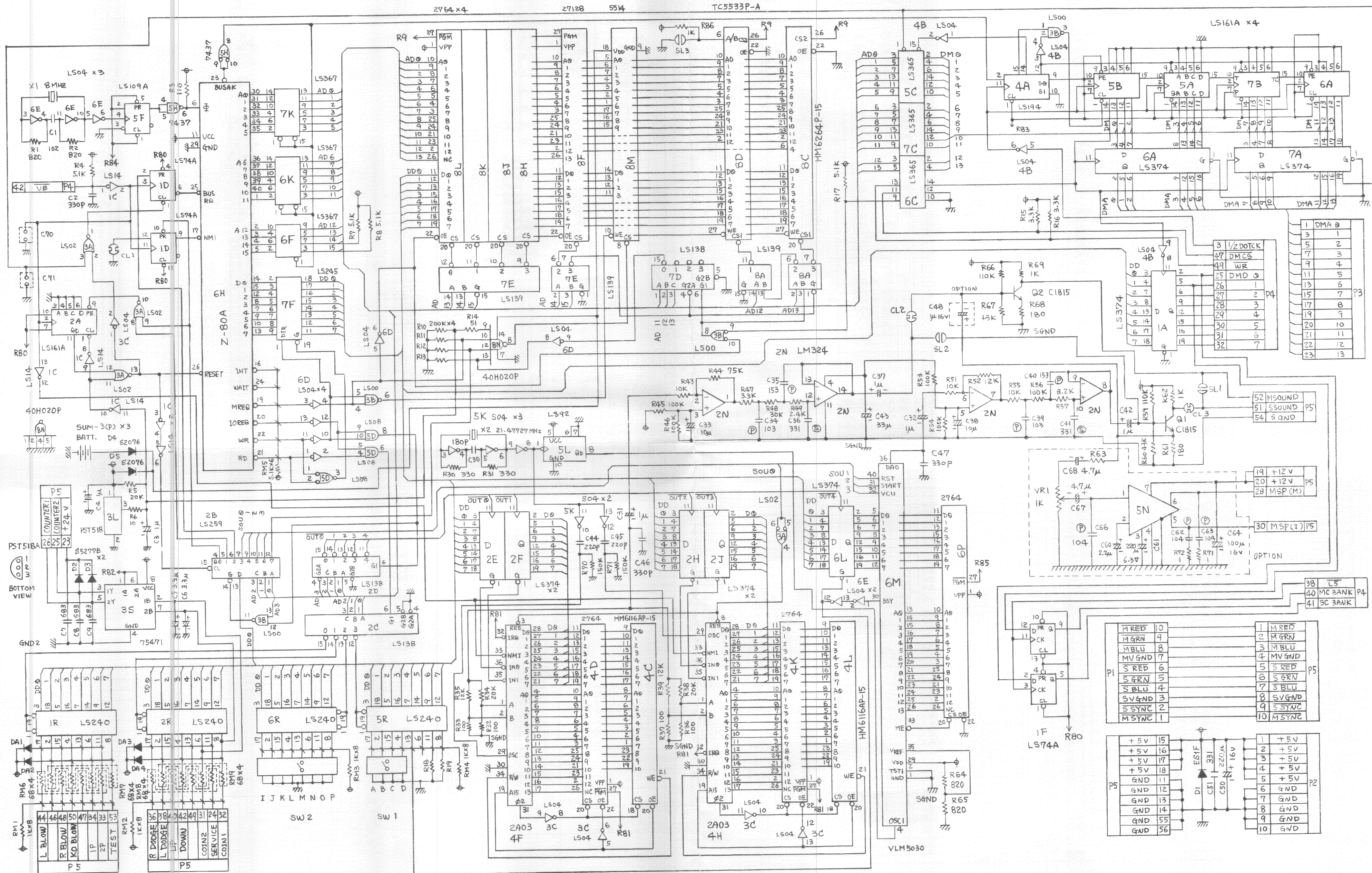
D CHP1-CPU SCHEMATIC ©1983 Nintendo of America Inc.
