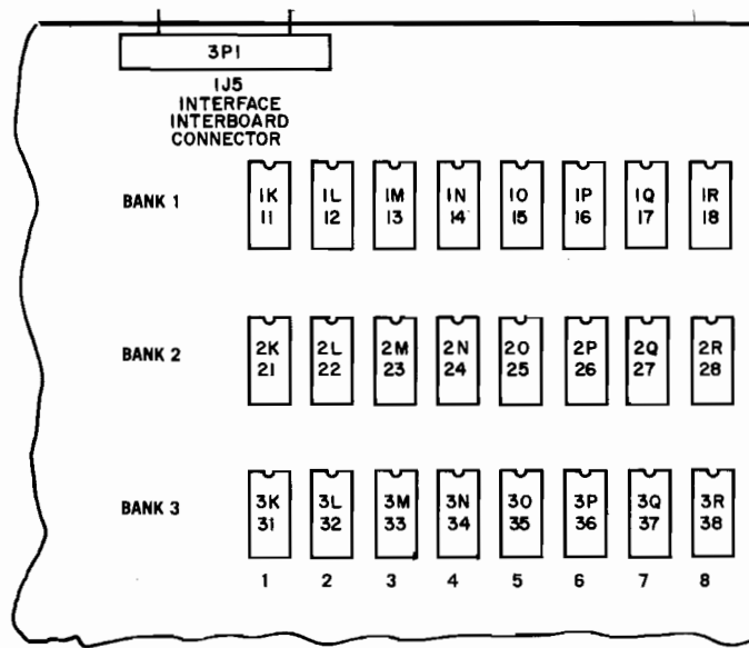
Figure 4. RAM Location and Numbering on CPU Board
