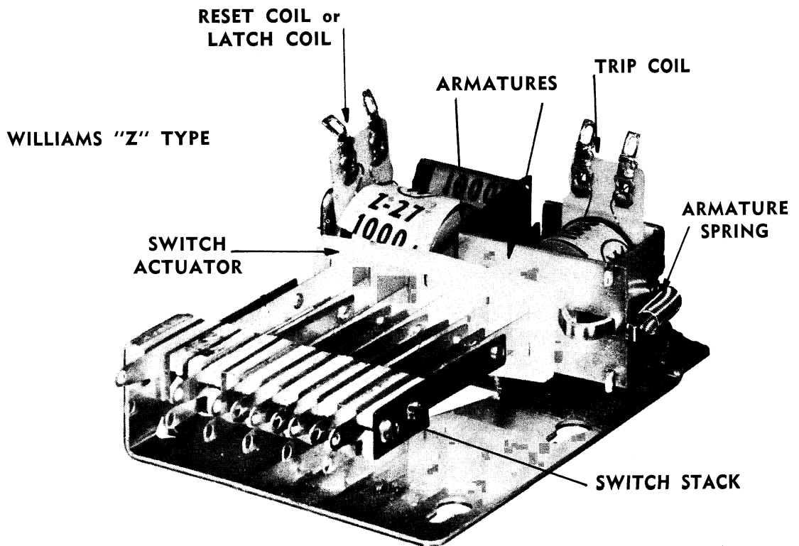
INTERLOCK RELAYS
