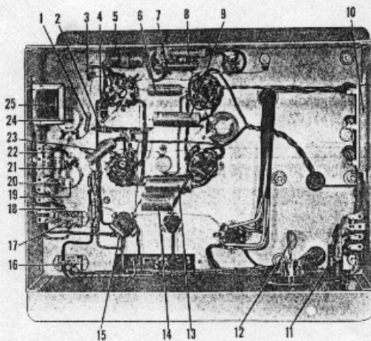
19790-A Amplifier Assembly (Less Tubes)
