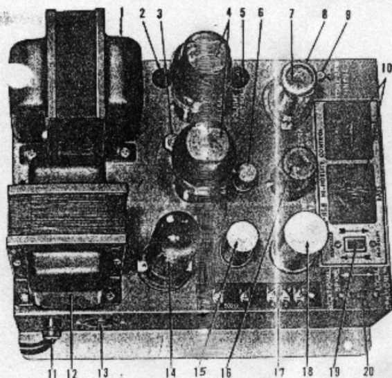
No. 19790-A Amplifier Assembly (Less Tubes)
