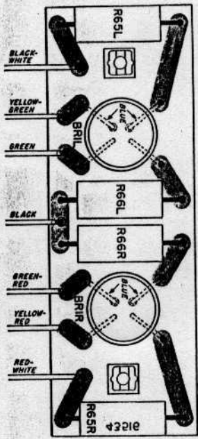
LAMP P.C. BOARD No. 4315-A (BARRETTERS)
