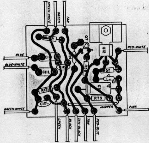
REGULATOR P.C. BOARD No. 440
