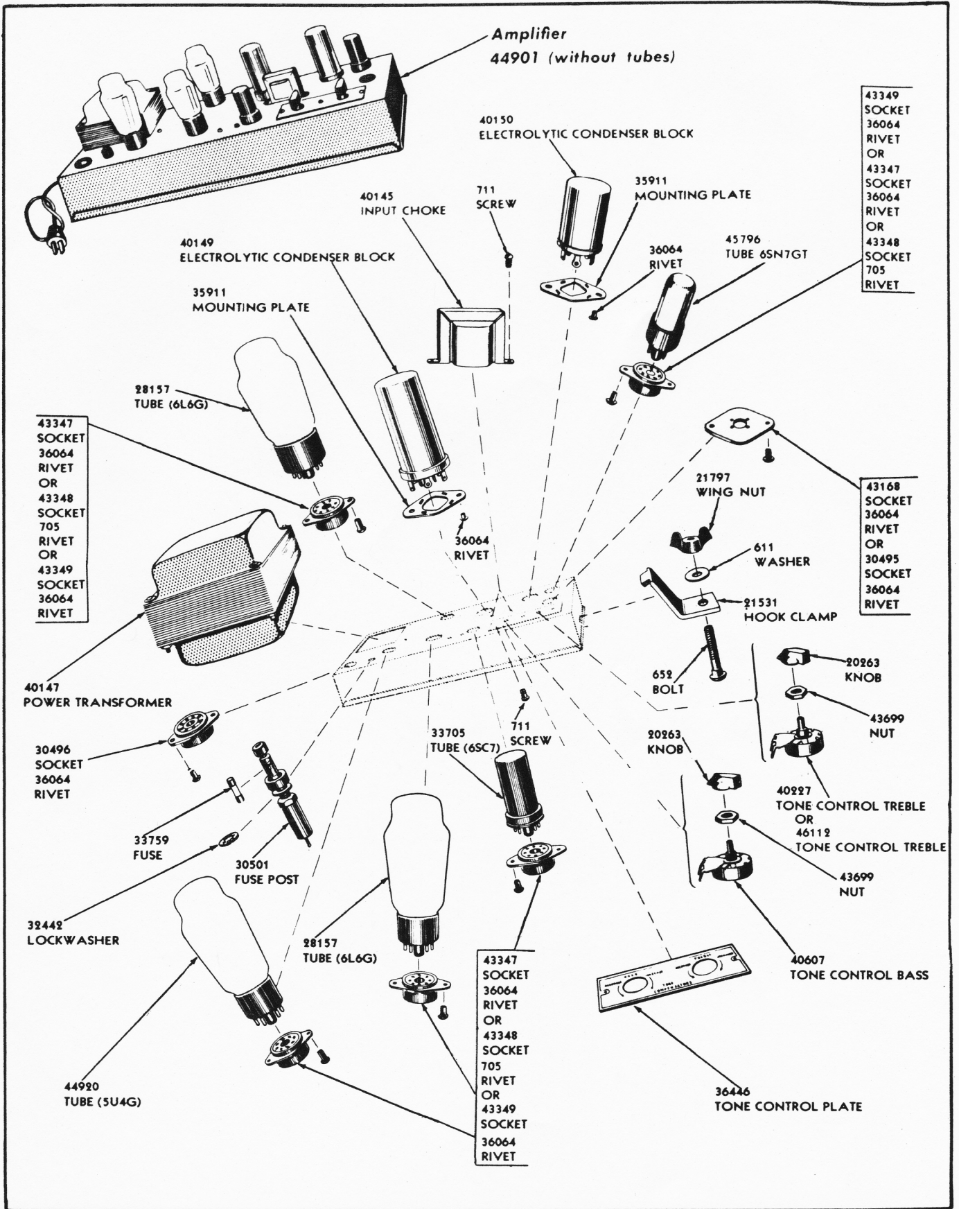
Figure 27—Model 503 Amplifier Sheet 1 of 2 Sheets
