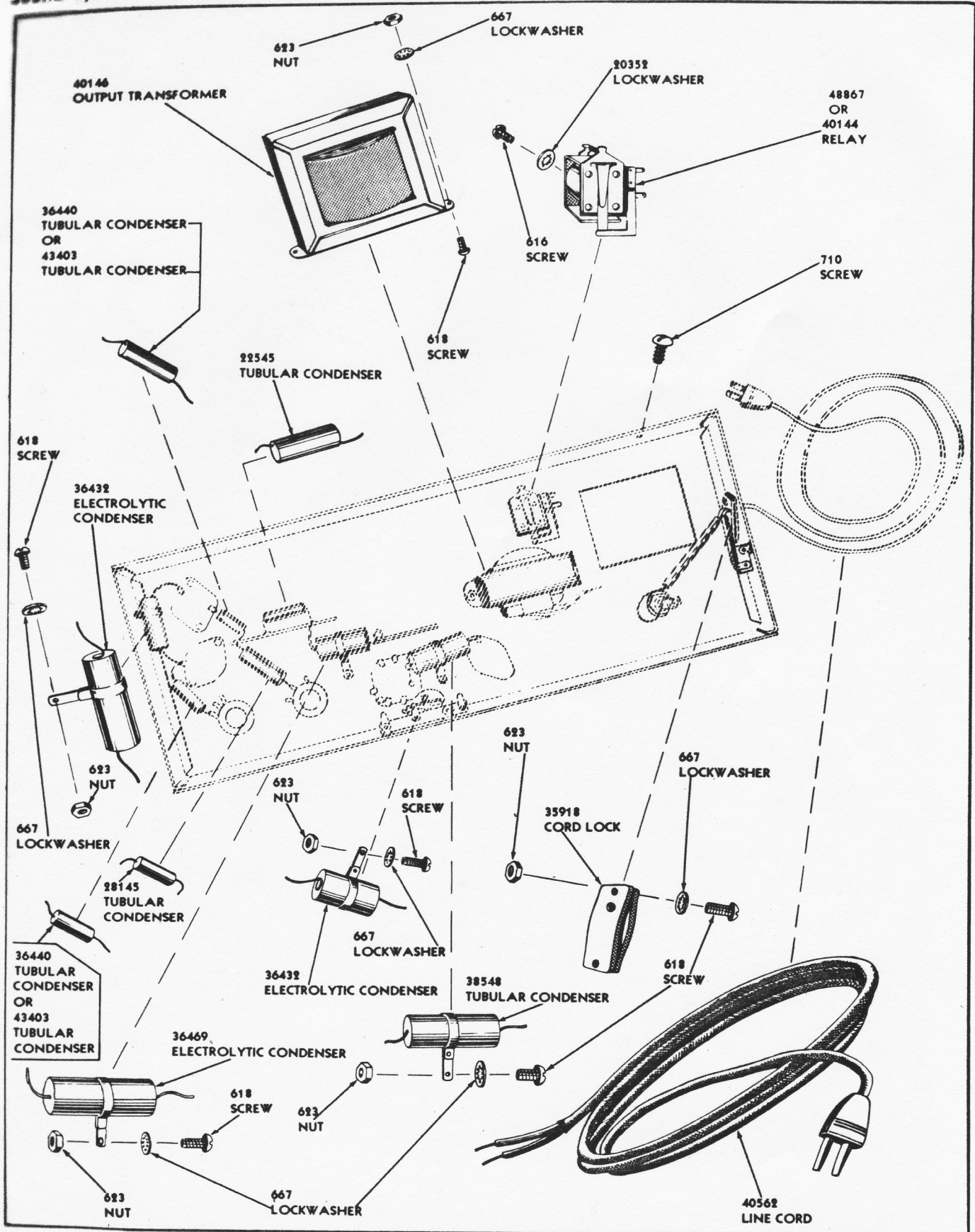
Figure 27—Model 503 Amplifier Sheet 2 of 2 Sheets
