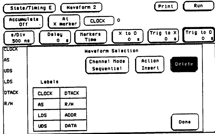
Figure 9-12. Delete Label
