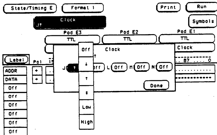
Figure 8-11. Negative-edge Selection
