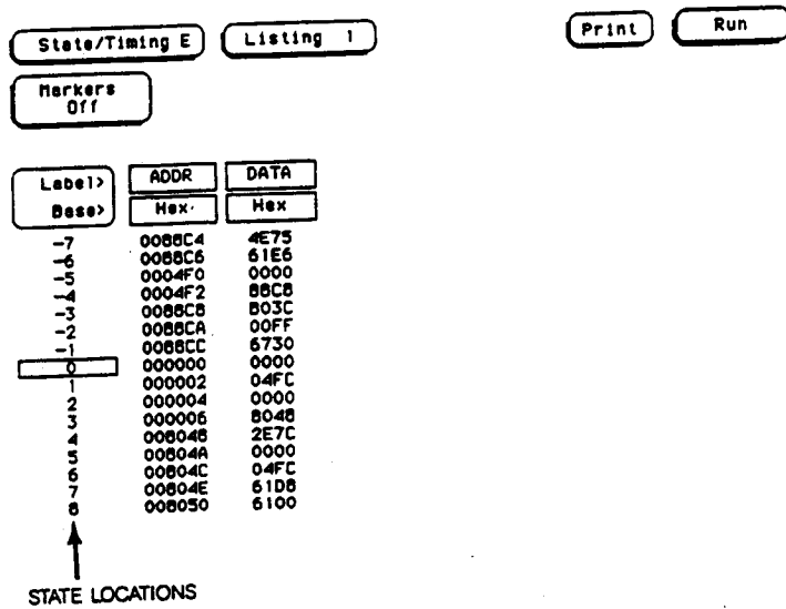
Figure 8-22. State Listing
