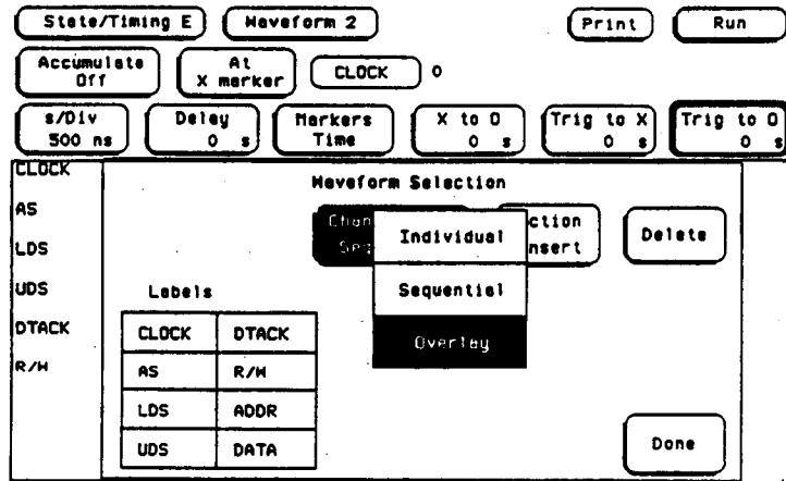
Figure 9-18. Overlay Selection
