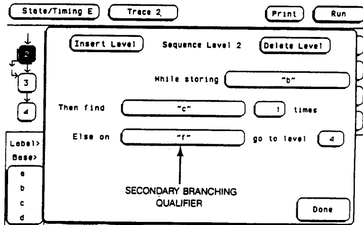
Figure 5-67. Secondary Branching
