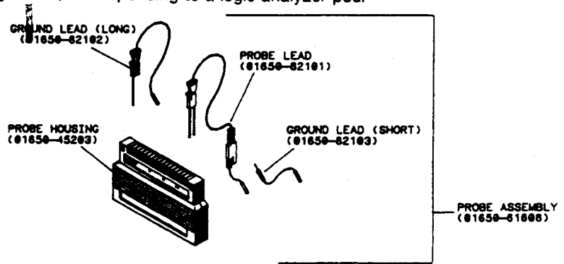
Figure 2-3. Probe Assembly
