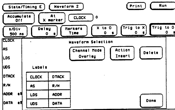
Figure 9-19. Overlapped Waveforms
