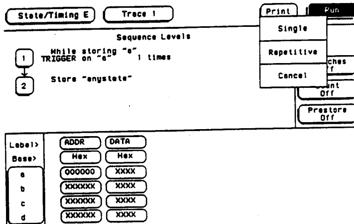
Figure 8-19. Acquiring Data
