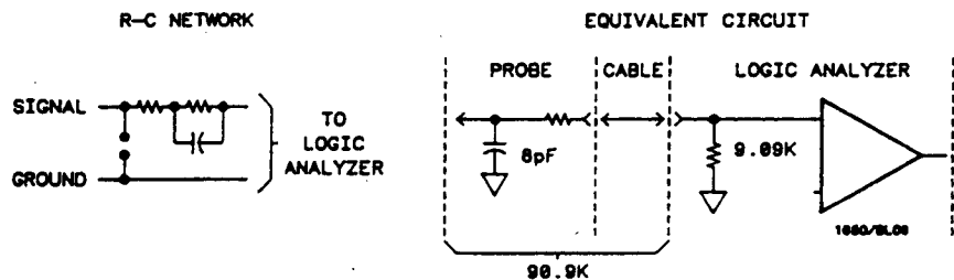
Figure 2-5. Probe Input Circuit
