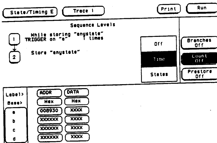
Figure 9-9. Count Time
