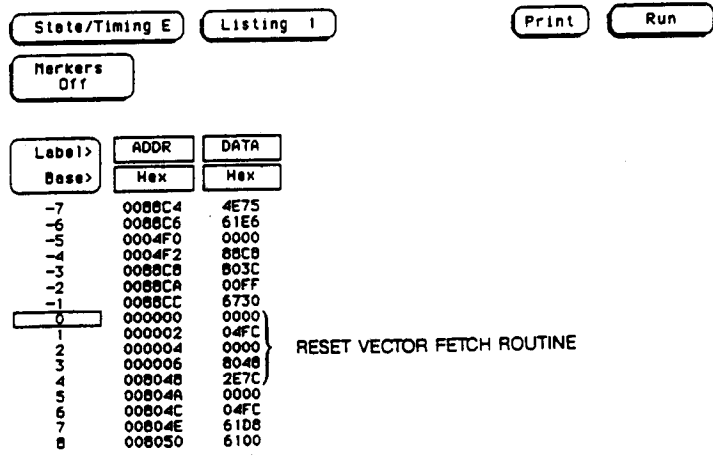
Figure 8-21. State Listing
